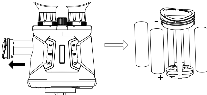
Figur 2-2 Installera batterier
