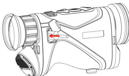
Figure 2-4 Connexion USB
